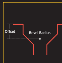
Countersunk Hole
